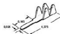
4 Solder Tab
