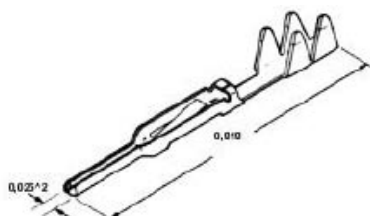
1 Pin Contact
